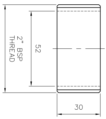
(SCALE-1:4) DETAIL-A BUSH FOR COUPLER
